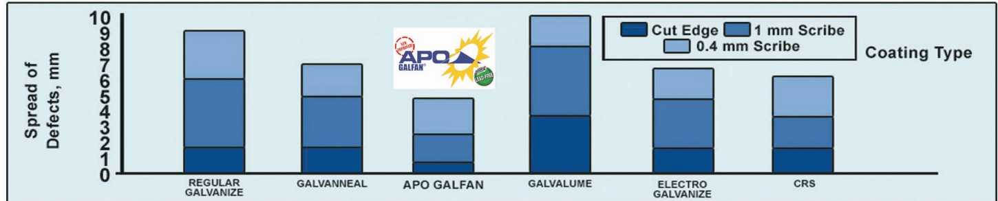
Figure 2 - Spread of defects after 2 years in industrial exposure.
